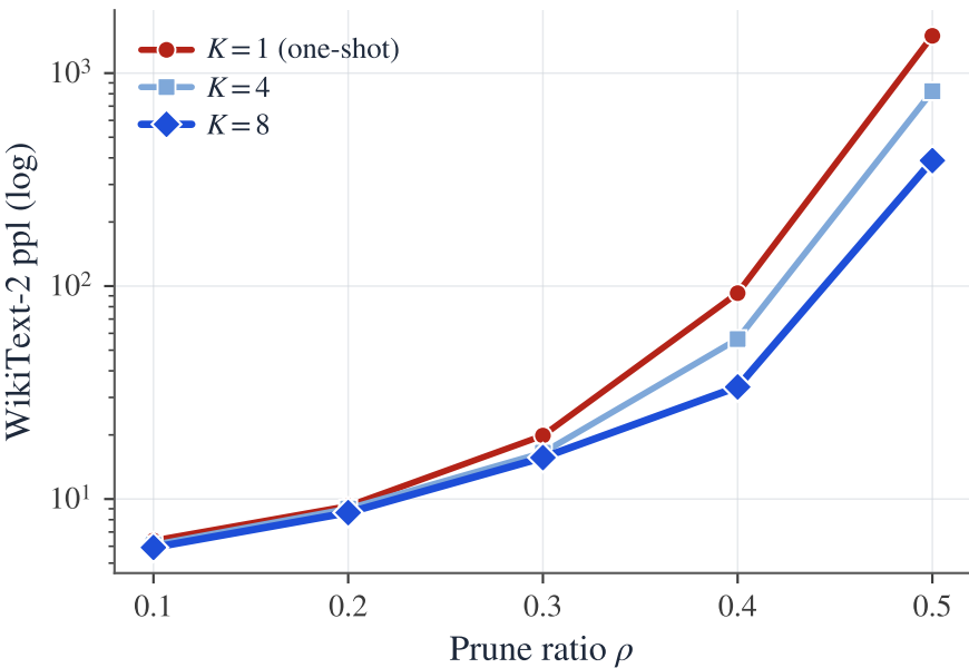
(a) Monotone in K (the 1/K^2 bound)
