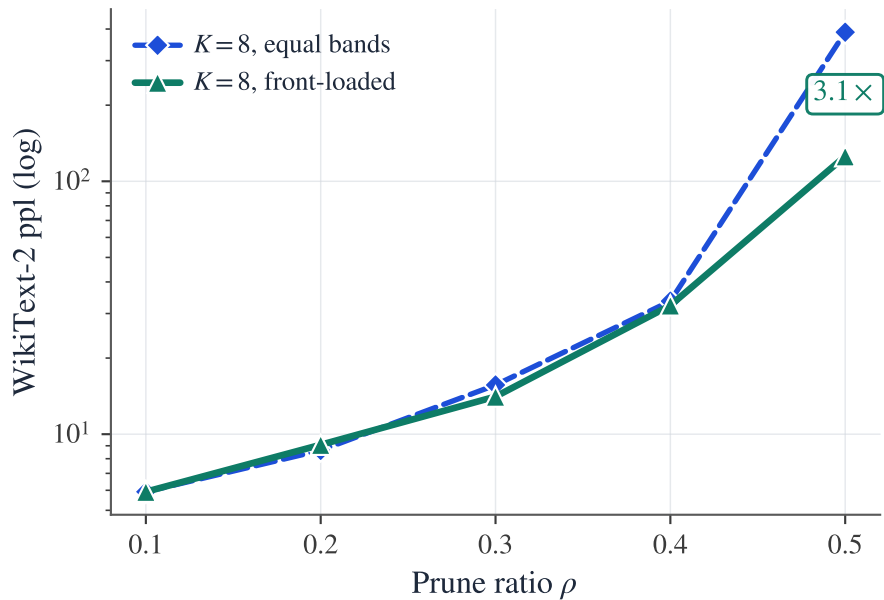
(b) Front-loading helps most where the path is steep
